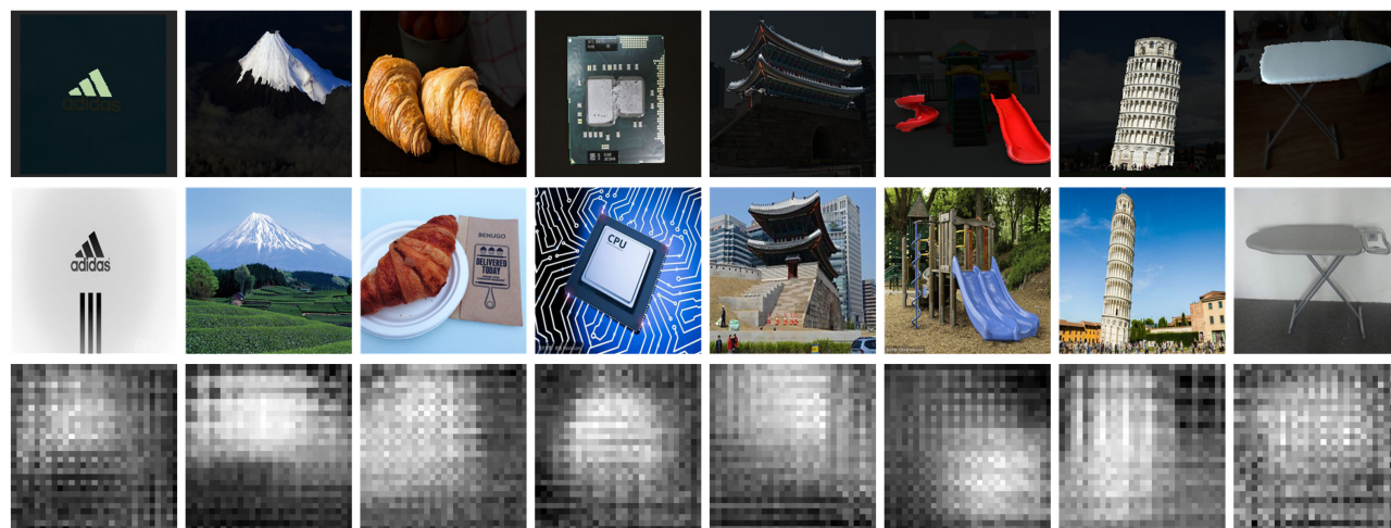
Fig. 13. Visual illustrations of prior masks for totally unseen objects in FSS-1000 dataset. Top : support images with the masked area in the target class. Middle : query images. Bottom : prior masks of query images where the regions of interest are highlighted.
