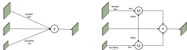
Fig. 10. Comparison between feature fusion strategies of (left) HRB and (right) HRB-Cond. Features from different scales are directly added to the main feature in (left), while in (right), essential information is selected from auxiliary features conditioned on the main features by the inter-scale merging module \mathcal{M} .
