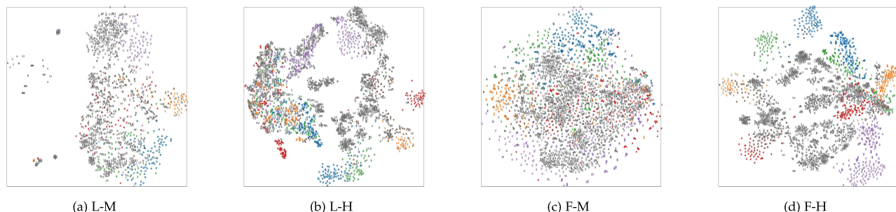
Fig. 12. Visual comparison between t-SNE results of different feature sources. 1,000 features in gray color are from base classes and 1,000 features in other colors are from novel classes. L-M : Learnable middle-level features. L-H : Learnable high-level features. F-M : Fixed middle-level features. F-H : Fixed high-level features.
