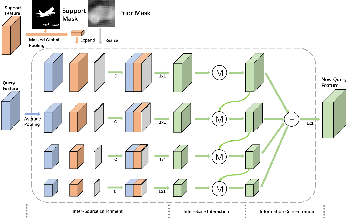
Fig. 4. Visual illustration of FEM (dashed box) with four scales and a top-down path. C, 1 \times 1 and Circled M represent concatenation, 1 \times 1 convolution and inter-scale merging module respectively. Activation functions are ReLU.
