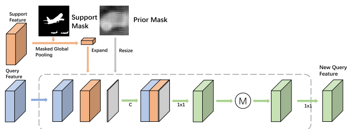
Fig. 6. Visual illustration of the baseline structure that processes features in the original spatial size of the input features.
