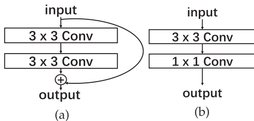
Fig. 7. Structures of (a) convolution block and (b) classification head.
