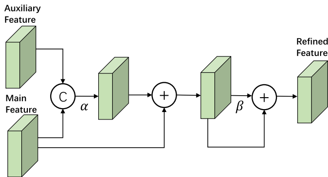
Fig. 5. Visual illustration of the inter-scale merging module \mathcal{M} . C is concatenation and + is pixel-wise addition. \alpha means 1 \times 1 convolution and \beta represents two 3 \times 3 convolutions. Activation functions are ReLU. For features that do not have auxiliary features, there is no concatenation with the auxiliary feature and the refined feature is produced only by the main feature with \alpha and \beta .
